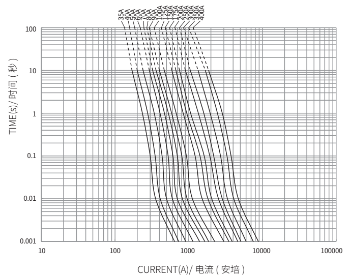
HBE 平均 I-T 曲线图 (仅供参考) AVERAGE I-T CHARACTERISTICS CURVE (FOR REFERENCE ONLY)
